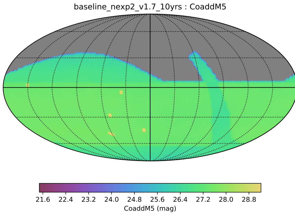
FIGURE 1: Example depth map from MAF, for the state of the survey at the conclusion of the 10 year baseline simulation.
